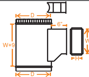
8. INJERTO ZAPATO RECTANGULAR
