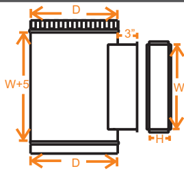
7. INJERTO RECTANGULAR
